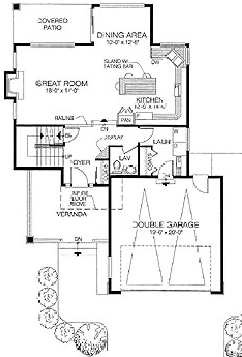
MAIN FLOOR PLAN 831 SQ. FT. (77.2 M 2 )
