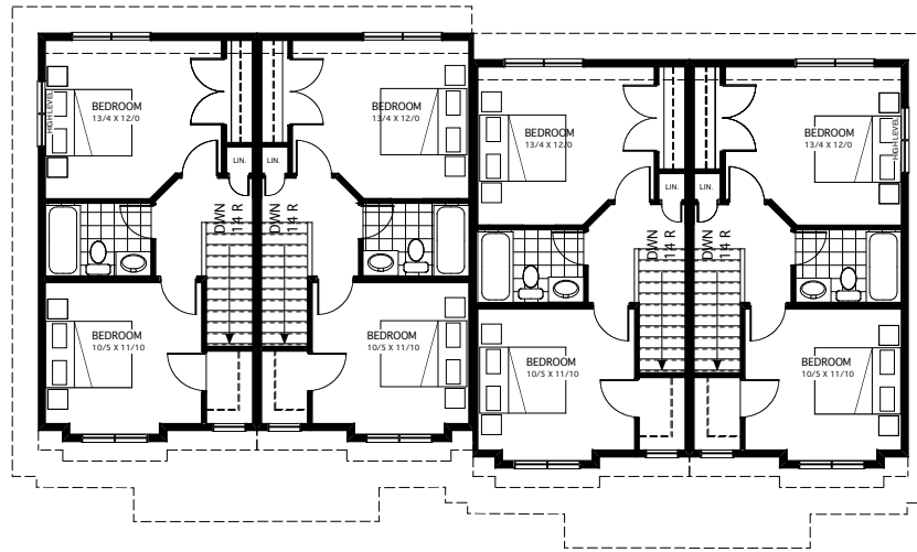
FOURPLEX UPPER FLOOR PLAN SCALE: 1/8" = 1'-0"
